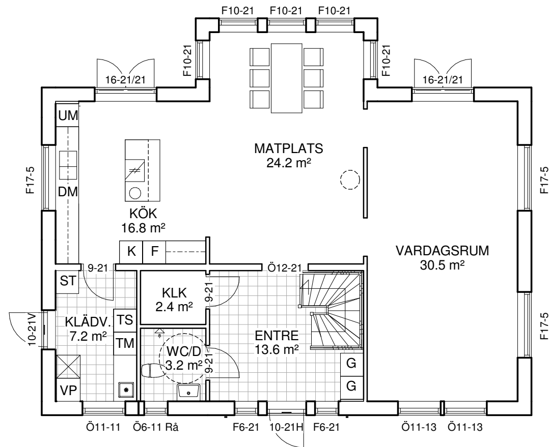
BOTTENPLAN
